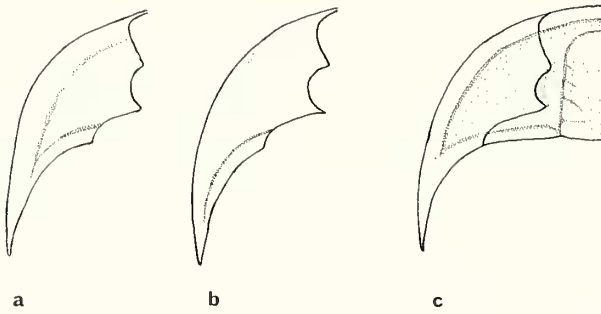
TEXT-FIG. 7. Dikelocephalacean genal structure to illustrate character 42 (see Table 2). Posterior border furrow continues into basal part at least of genal spine. a , cheek of typical saukiid with defined, gently convex lateral border. b , in Dikelocephalidae lateral border is generally flattened, but characteristic furrow usually remains defined. c , primitive ptychoparioid condition. All approximately natural size.
